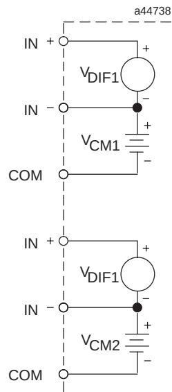
Figure 9-3. Analog Input Common Mode Voltage
