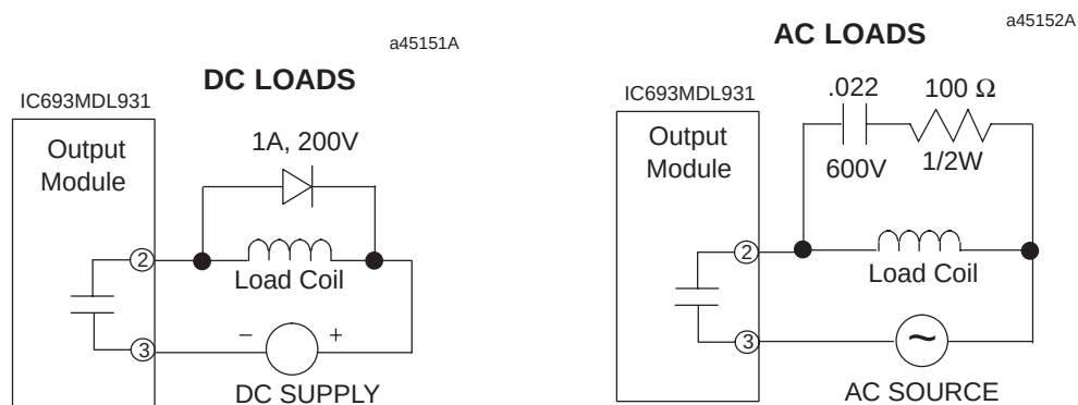
Figure 7-33. Load Suppression Examples for IC693MDL931 Output Module
