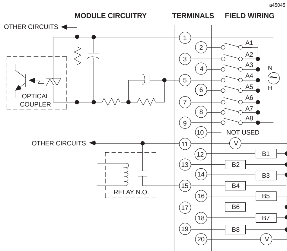
Figure 8-1. Field Wiring 120 VAC Input/Relay Output Module - IC693MAR590
