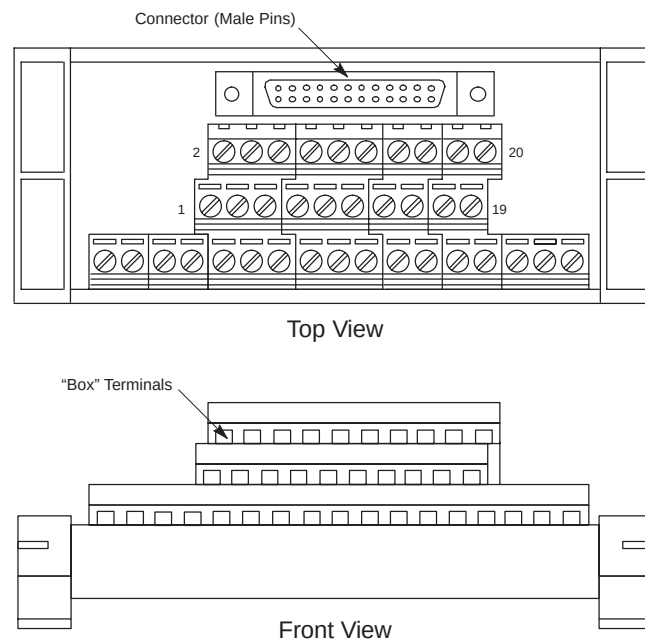
Figure C-1. Typical TBQC Terminal Block
