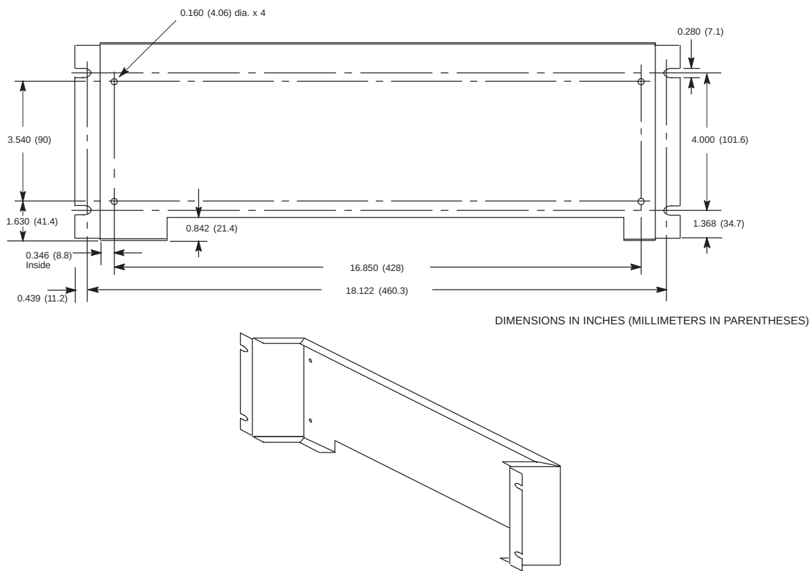
Figure 3-20. IC693ACC313 Recessed Mount Adapter Bracket
