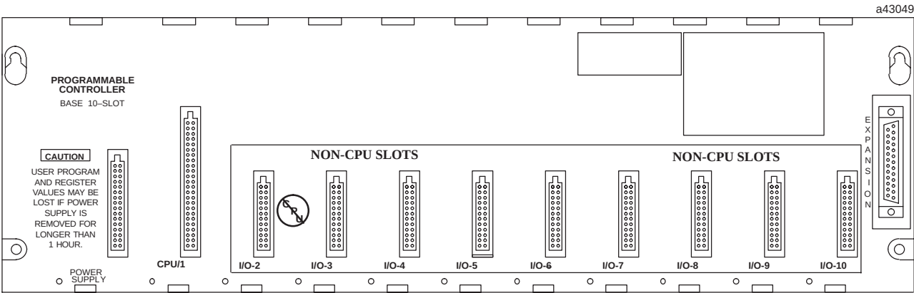
Figure 3-5. IC693CHS391 10-Slot Modular CPU Baseplate
