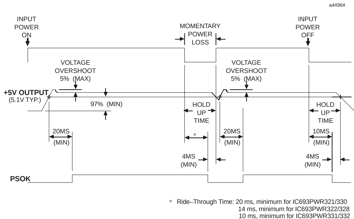
Figure 4-14. Timing Diagram for all Series 90-30 Power Supplies
