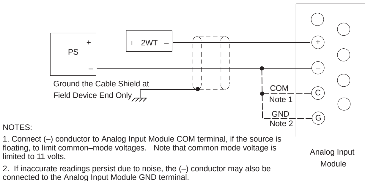
Figure 2-19. 2-Wire Transducer, Externally Powered via DC Supply
