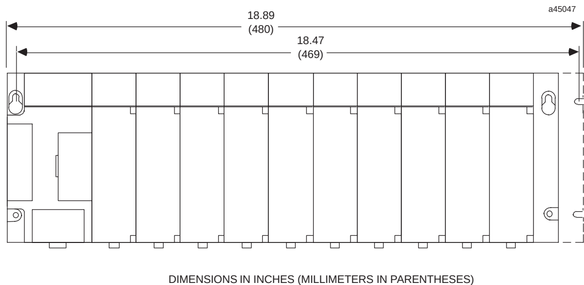
Figure 3-19. Dimensions for 19" Rack Mounting Using IC693ACC308 Adapter Bracket
