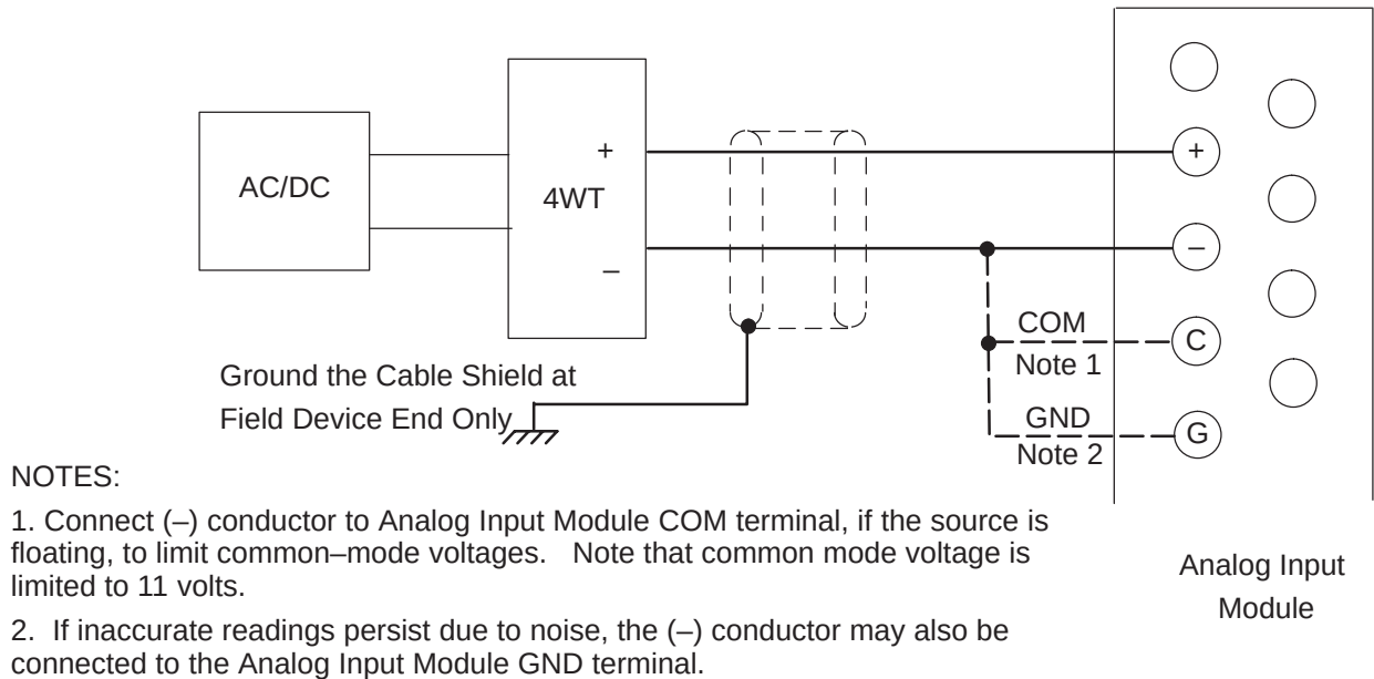
Figure 2-18. 4-Wire Transducer, Externally Powered via AC or DC Supply
