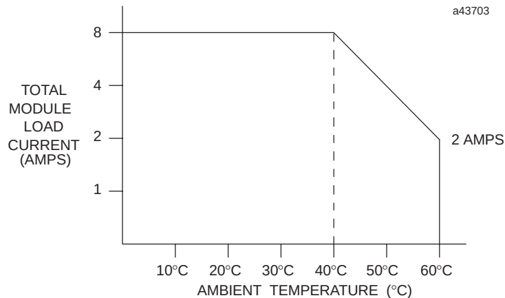
Figure 7-5. Input Points vs. Temperature for IC693MDL330
