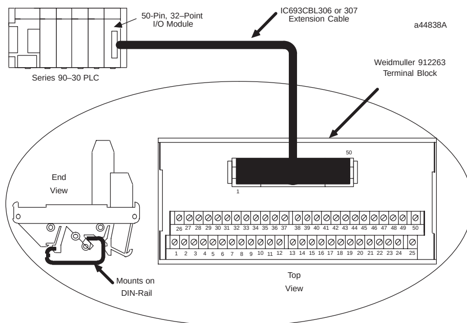
Figure 2-13. 50-PIN I/O Module with Weidmuller #912263 Terminal Block
