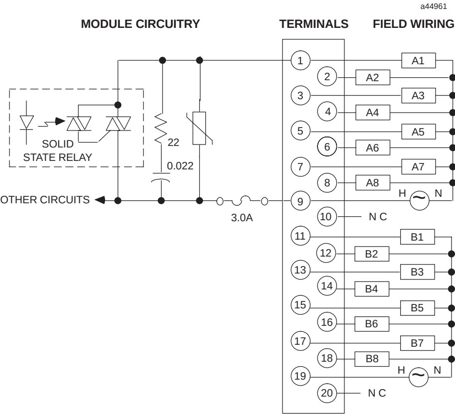
Figure 7-6. IC693MDL340 Output Module Field Wiring
