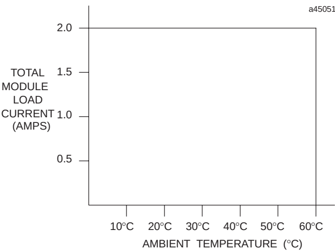
Figure 7-19. Load Current vs. Temperature for IC693MDL733
