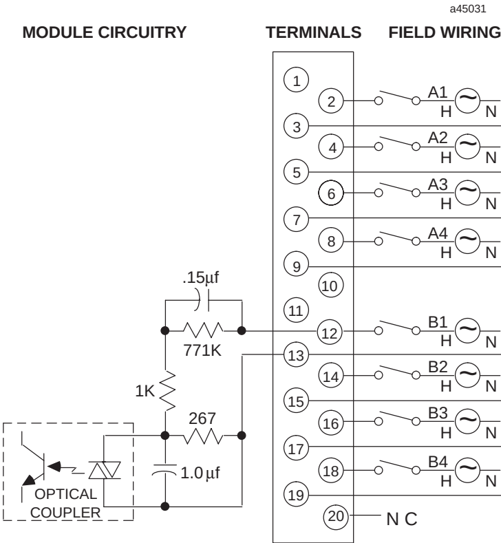
Figure 6-2. Field Wiring - 240 Volt AC Isolated Input Module - IC693MDL231
