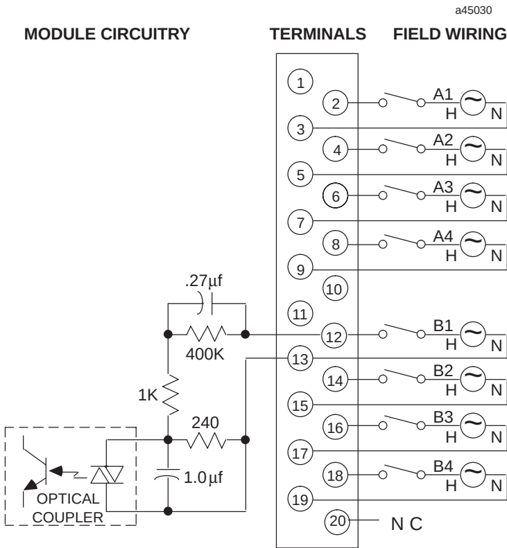
Figure 6-1. Field Wiring - 120 Volt AC Isolated Input Module - IC693MDL230
