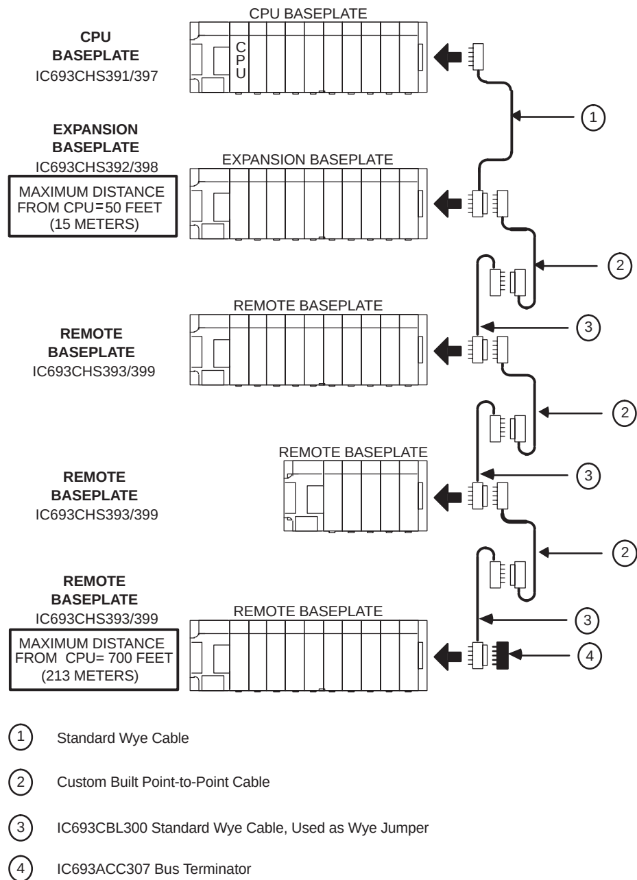
Figure B-8. Example of Connecting Expansion and Remote Baseplates
