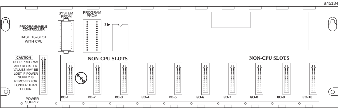
Figure 3-3. IC693CPU323 10-slot Embedded CPU Baseplate
