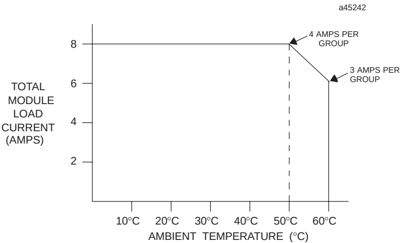
Figure 7-27. Load Current vs. Temperature for IC693MDL742
