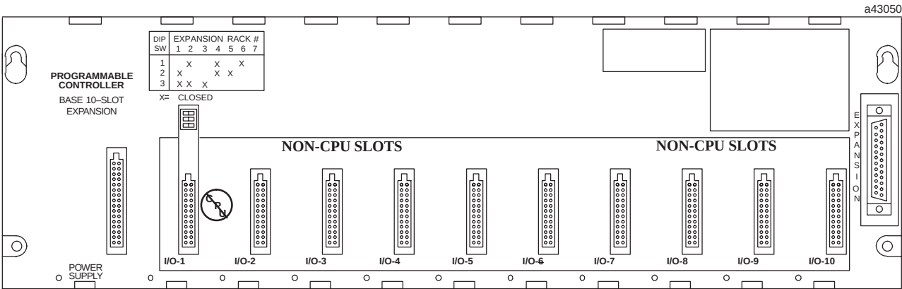
Figure 3-7. IC693CHS392 10-Slot Expansion Baseplate
