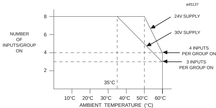
Figure 6-19. Input Points vs. Temperature for IC693MDL655
