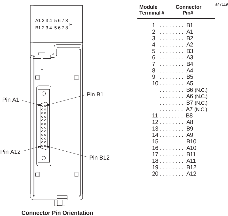
Figure C-2. IC693ACC334 TBQC Faceplate
