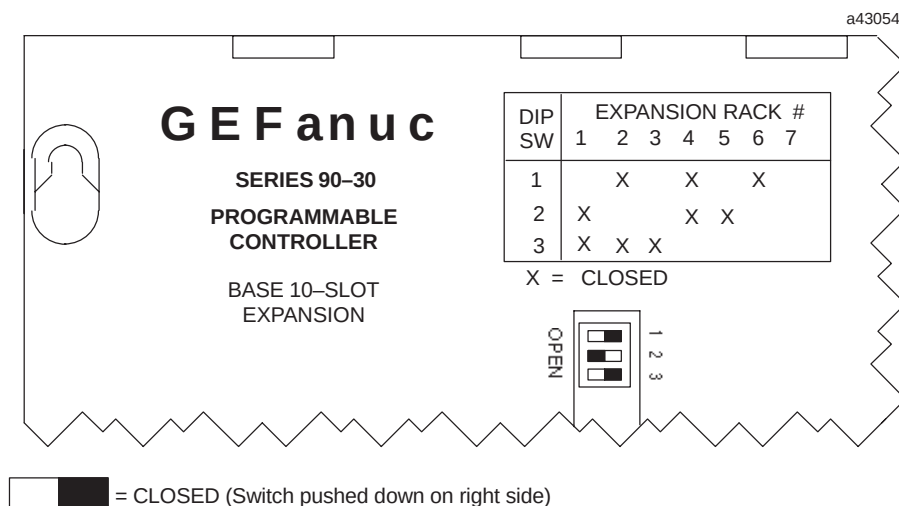
Figure 3-11. Rack Number Selection Switch (Shown with Rack 2 Selected)
