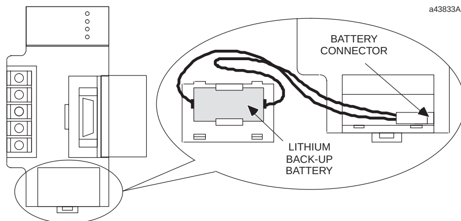
Figure 4-16. Backup Battery for RAM Memory
