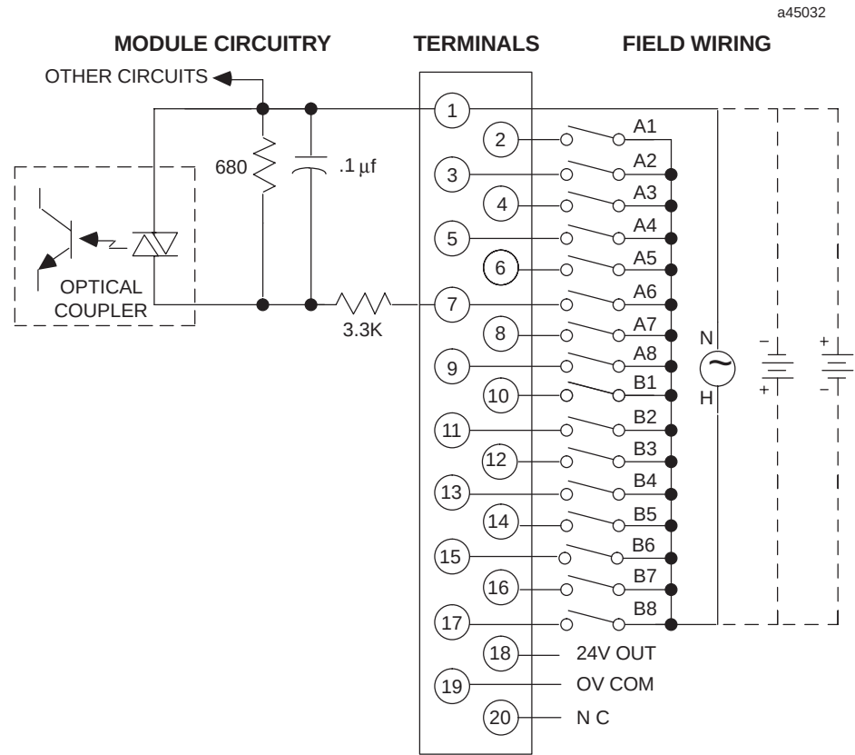
Figure 6-5. Field Wiring - 24 Volt AC/DC Pos/Neg Logic Input Module - IC693MDL241
