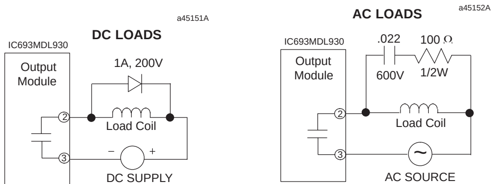
Figure 7-30. Load Suppression Examples for IC693MDL930 Output Module
