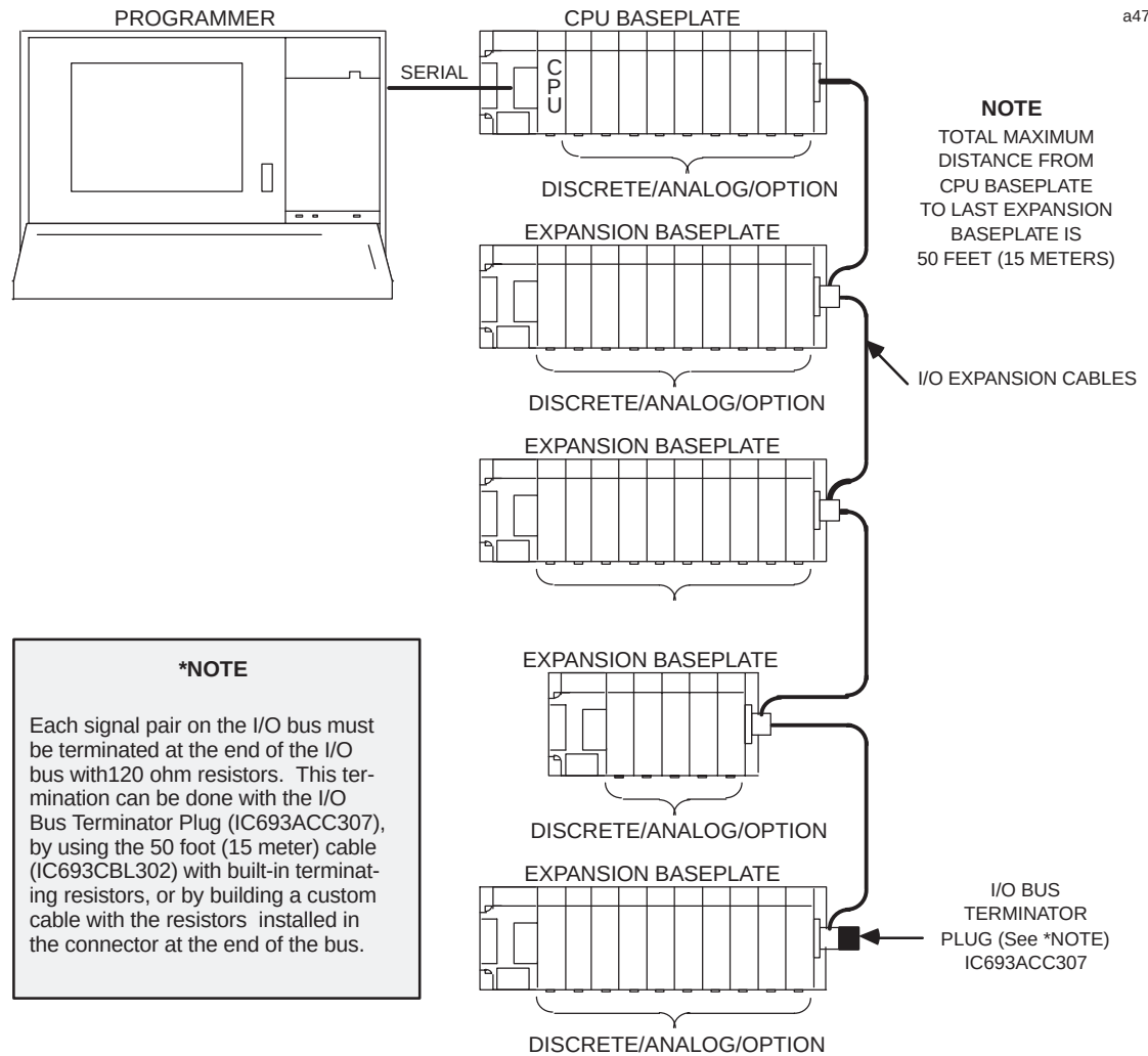
Figure 3-12. Example of Connecting Expansion Baseplates
